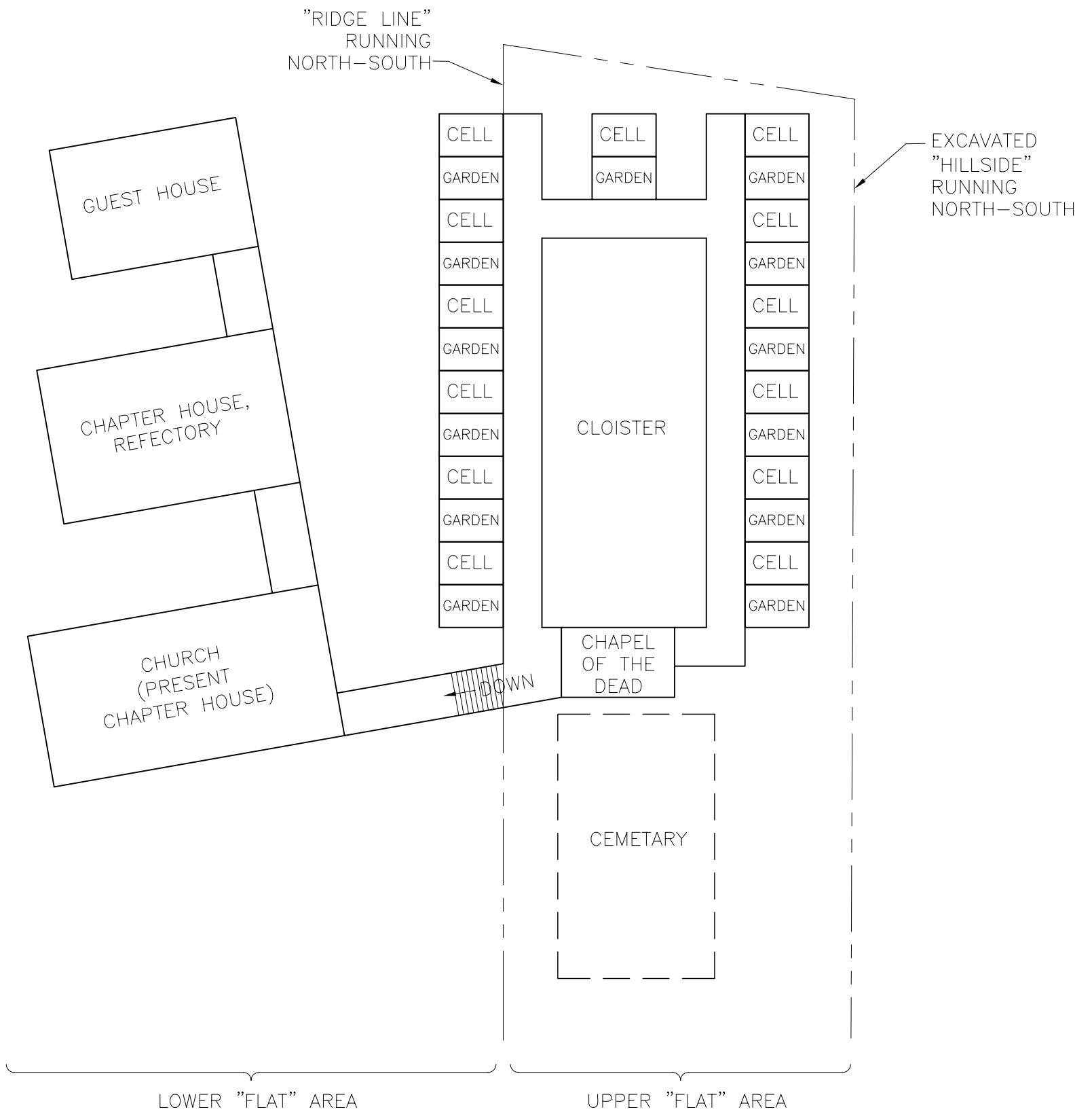
PLAN VIEW
